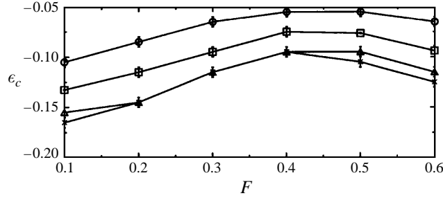
FIGURE 16. Onset \epsilon as a function of F in one dimension \psi_1 = 0.025 and B = 18 ( \circ ), B = 30 ( \square ), B = 67 ( \triangle ), B = 100 ( \times ).
